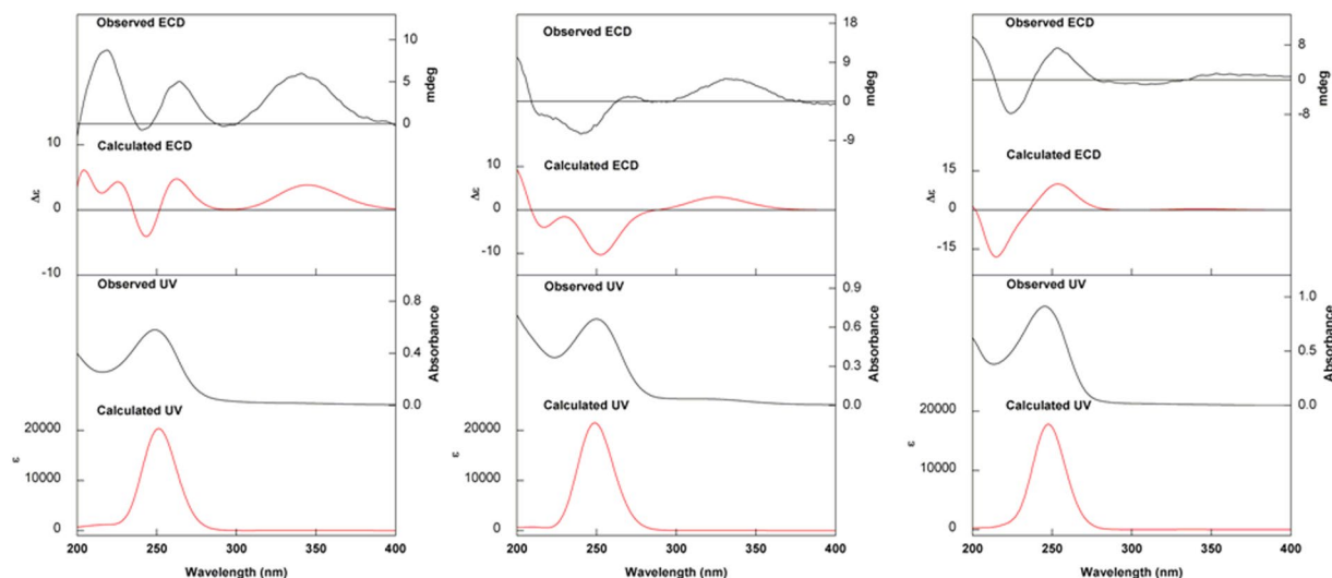
Figure 5. (Left) Experimental and calculated [2R,4R,5R,8S; CAM-B3LYP/PCM(MeOH)/TZVP//B3LYP/PCM(MeOH)/6-31G(d)] UV and ECD spectra of (+)- 2 (Center) Experimental and calculated [2R,4S,5R,8R; CAM-B3LYP/PCM(MeOH)/TZVP//B3LYP/PCM(MeOH)/6-31G(d)] UV and ECD spectra of (+)- 3 (Right) Experimental and calculated [2R,4R,8R; CAM-B3LYP/PCM(MeOH)/TZVP//B3LYP/PCM(MeOH)/6-31G(d)] UV and ECD spectra of (+)- 4 . For structures of the lowest-energy conformers, please see Supplementary Information.
