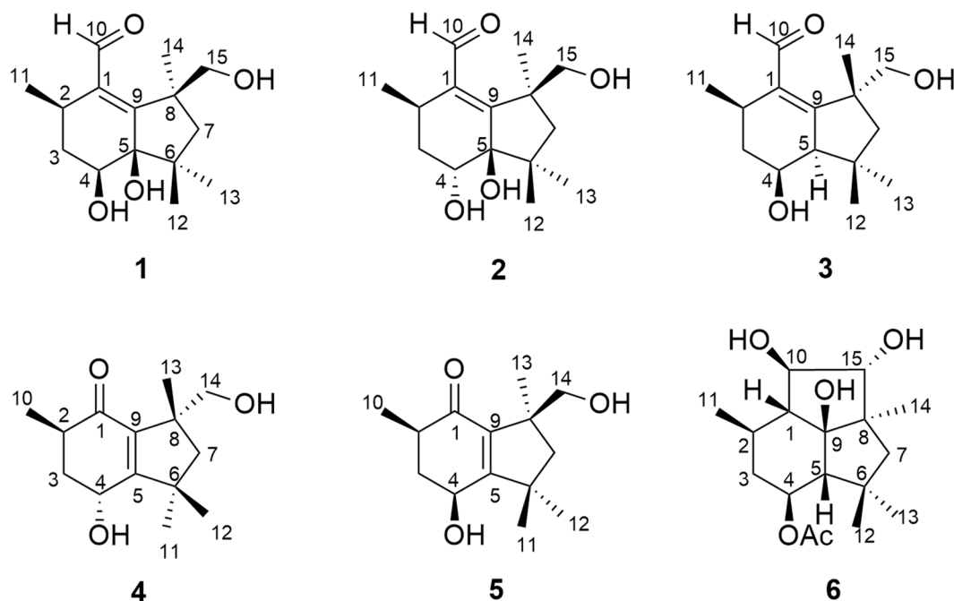
Figure 1. Botryane terpenoids isolated from EtOAc extract of Nemanja bipapillata cultures.
